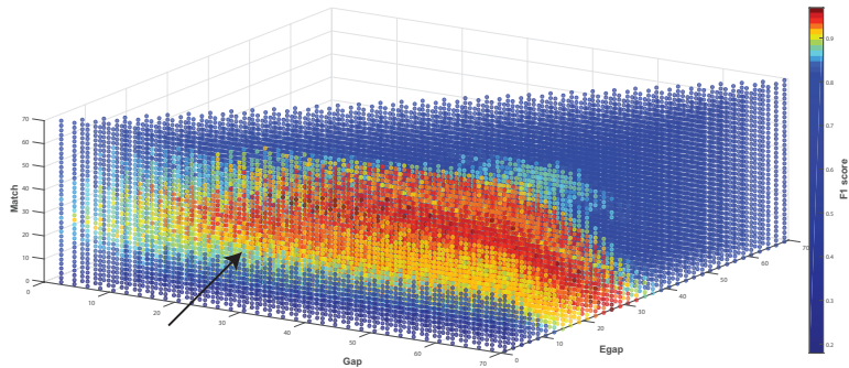
Figure 5: Exhaustive performance evaluation conducted on the parameter space ( match x gap x egap ). Colours show F1 scores: dark blue shades show low to average scores, whereas light blue to brown shades show high scores, i.e. > 0.85 . Performance of the selected parameters is indicated by the black arrow.
